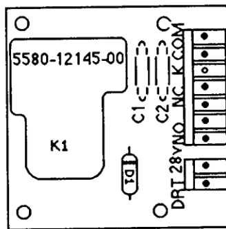
Motor Relay Board Assembly p/n C-11902-1
