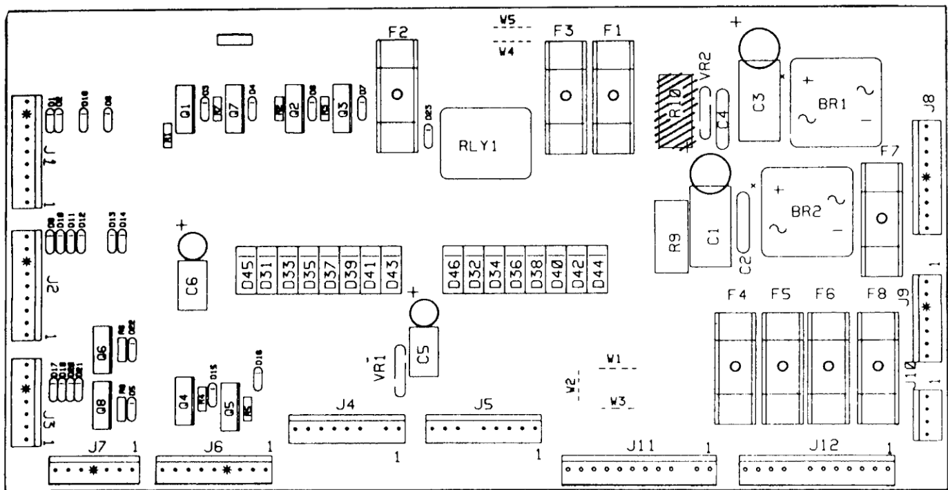
Aux Power Driver Unit Board p/n D-11813-552
